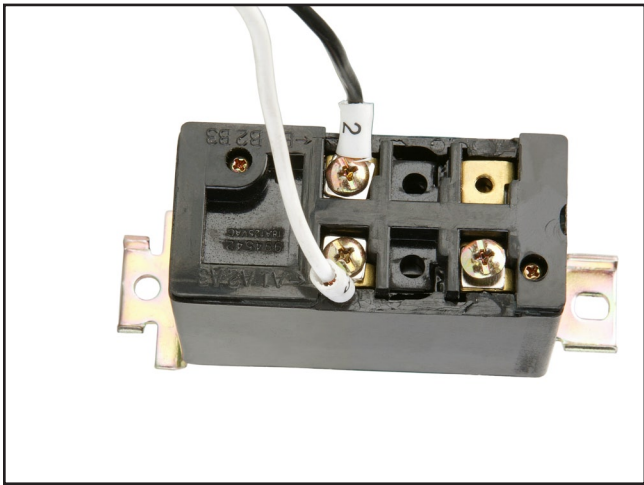
Figure 71. ON/OFF switch.
